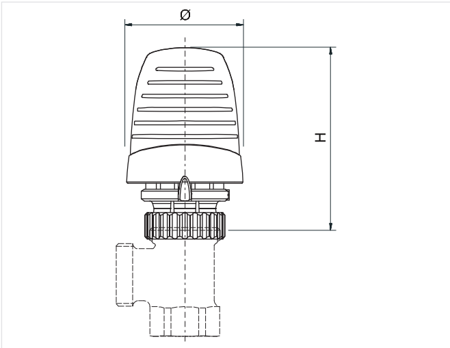
Fig. 1 Tera-4 Classic with internal sensor
