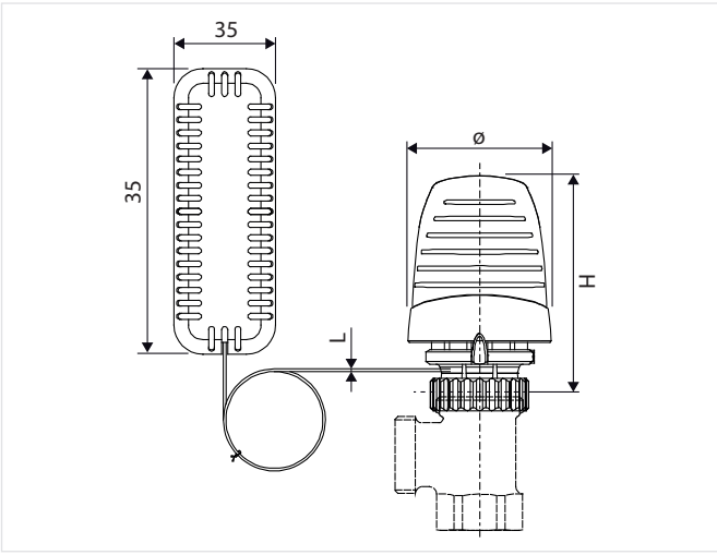
Fig. 2 Tera-4 Classic with remote sensor
